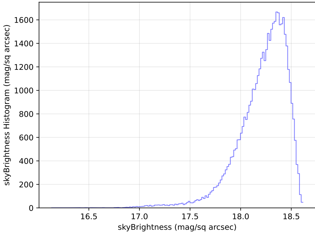
too_elab_heavy_r128_d3_ugrizy_v3.4_10yrs Yr 1 y band: skyBrightness Histogram
