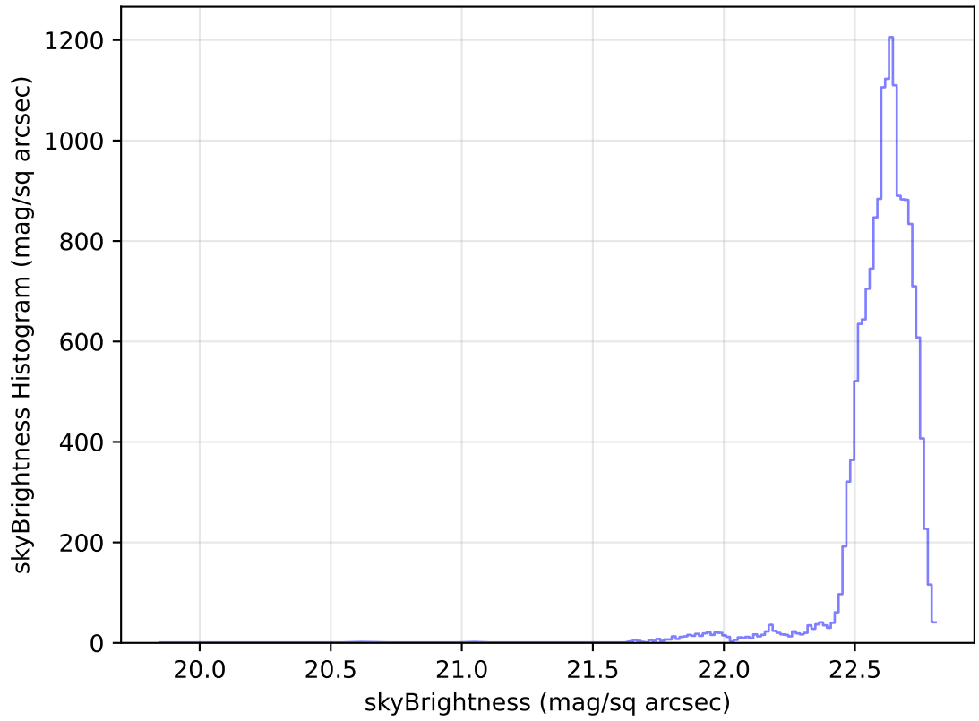
too_elab_heavy_r128_d3_ugrizy_v3.4_10yrs Yr 1 u band: skyBrightness Histogram
