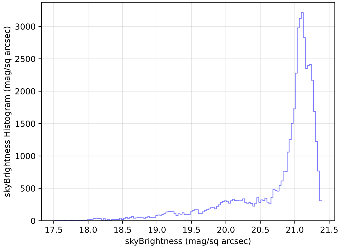
too_elab_heavy_r128_d3_ugrizy_v3.4_10yrs Yr 1 r band: skyBrightness Histogram
