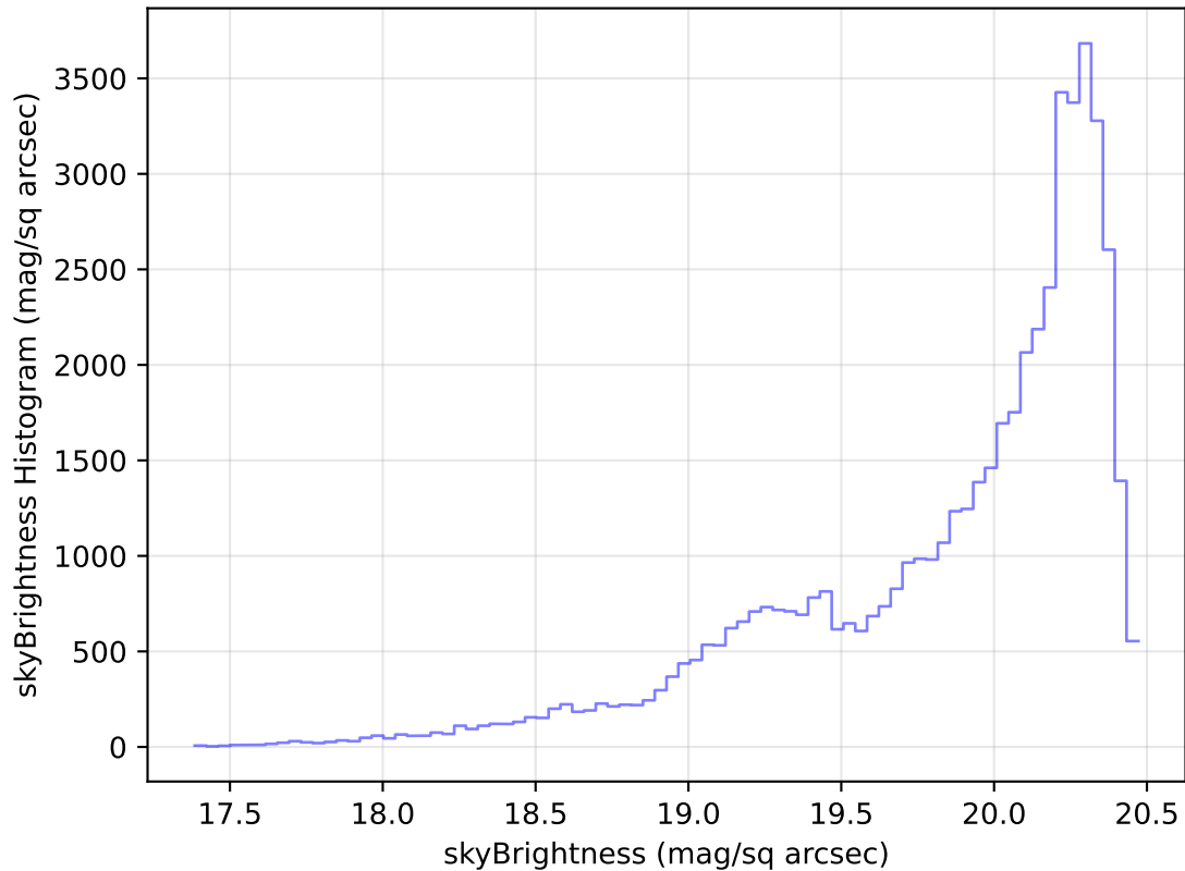
too_elab_heavy_r128_d3_ugrizy_v3.4_10yrs Yr 1 i band: skyBrightness Histogram
