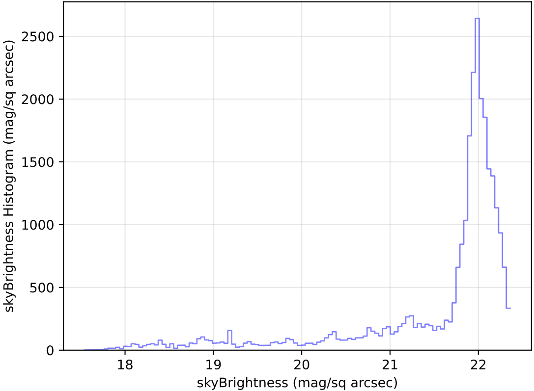
too_elab_heavy_r128_d3_ugrizy_v3.4_10yrs Yr 1 g band: skyBrightness Histogram
