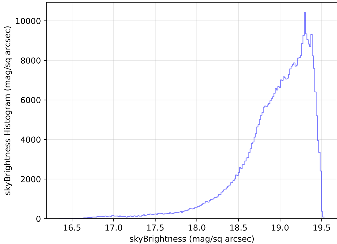
too_elab_heavy_r128_d3_ugrizy_v3.4_10yrs WFD z band: skyBrightness Histogram
