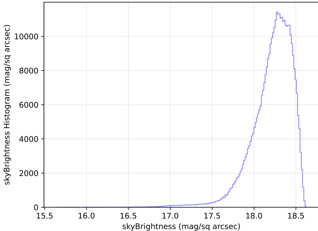
too_elab_heavy_r128_d3_ugrizy_v3.4_10yrs WFD y band: skyBrightness Histogram
