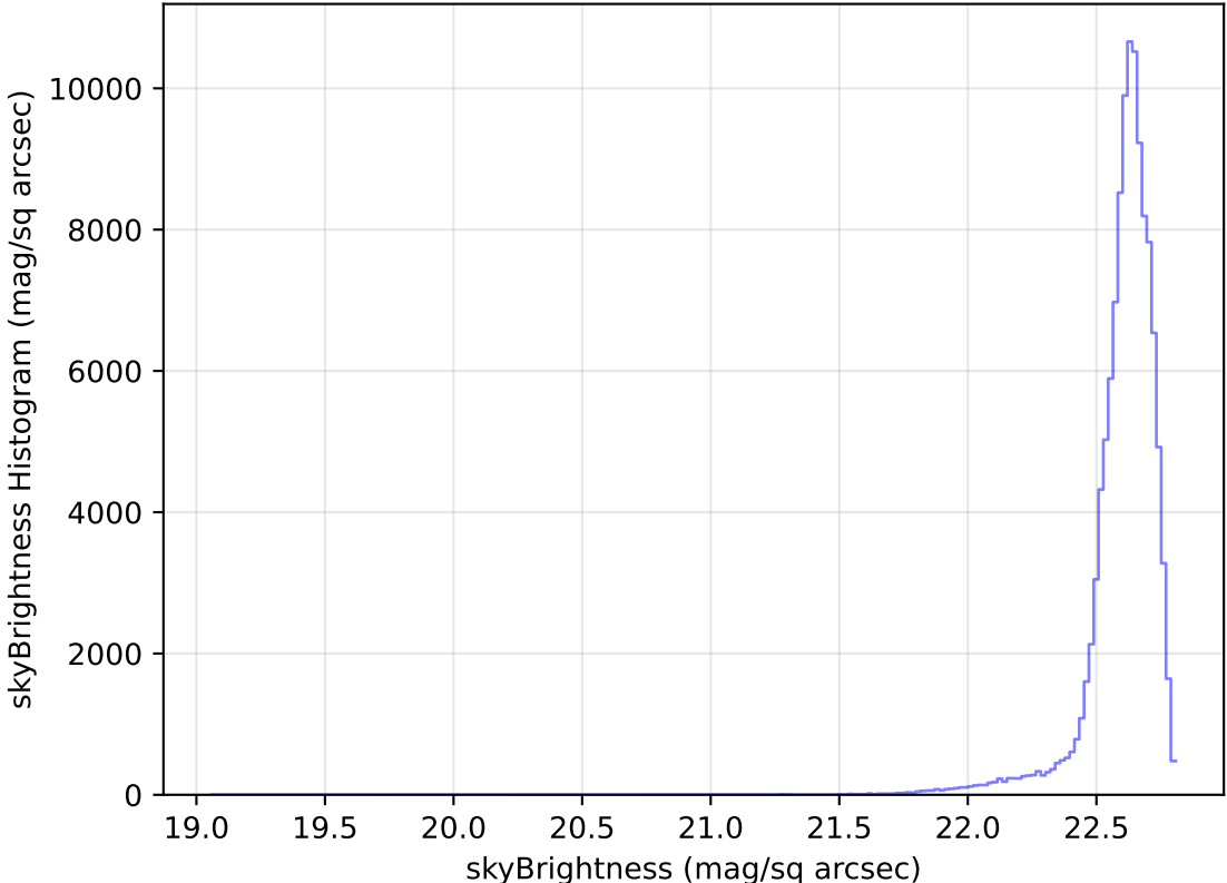
too_elab_heavy_r128_d3_ugrizy_v3.4_10yrs WFD u band: skyBrightness Histogram
