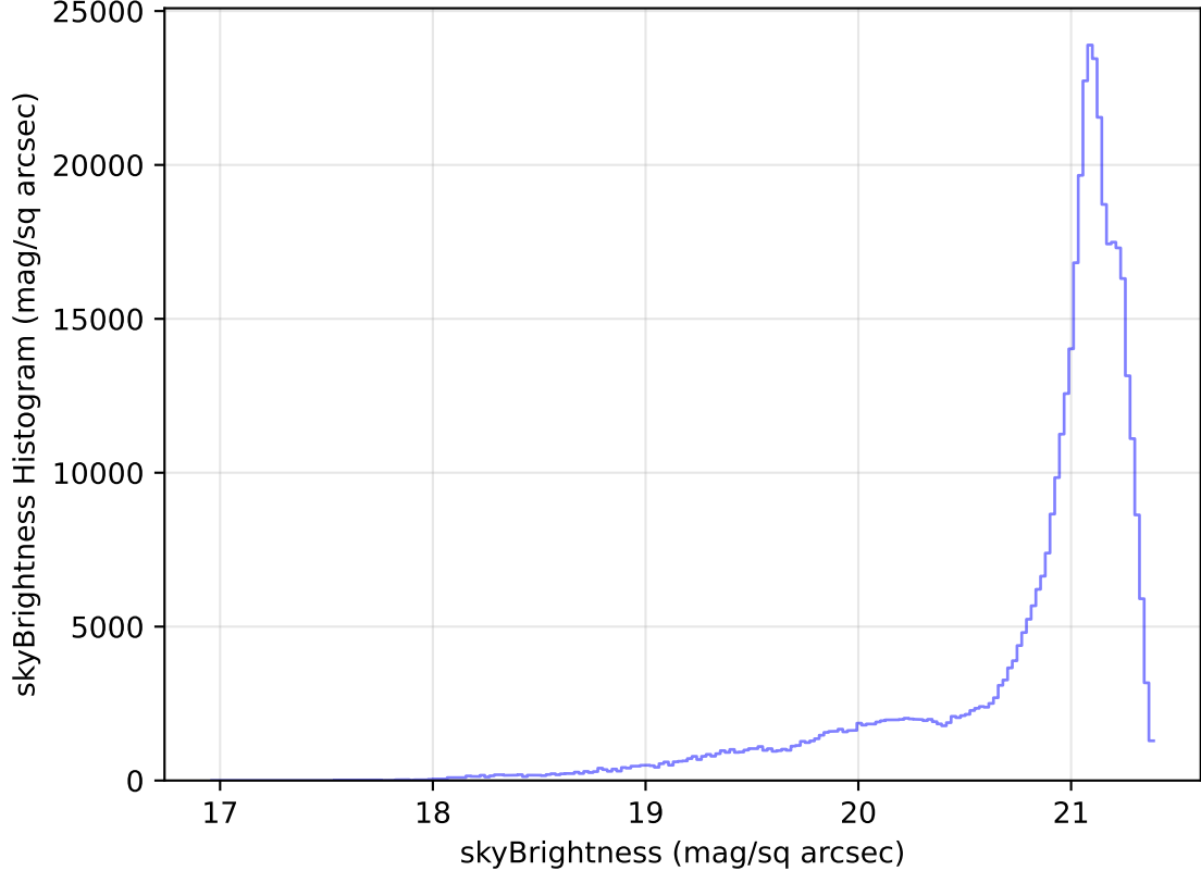
too_elab_heavy_r128_d3_ugrizy_v3.4_10yrs WFD r band: skyBrightness Histogram
