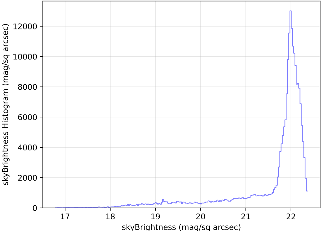
too_elab_heavy_r128_d3_ugrizy_v3.4_10yrs WFD g band: skyBrightness Histogram
