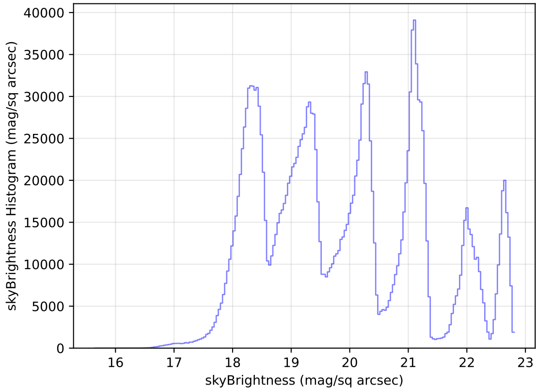
too_elab_heavy_r128_d3_ugrizy_v3.4_10yrs WFD all bands: skyBrightness Histogram
