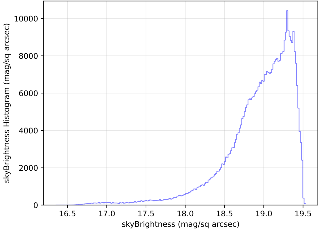
too_elab_heavy_r128_d3_ugrizy_v3.4_10yrs All sky z band: skyBrightness Histogram
