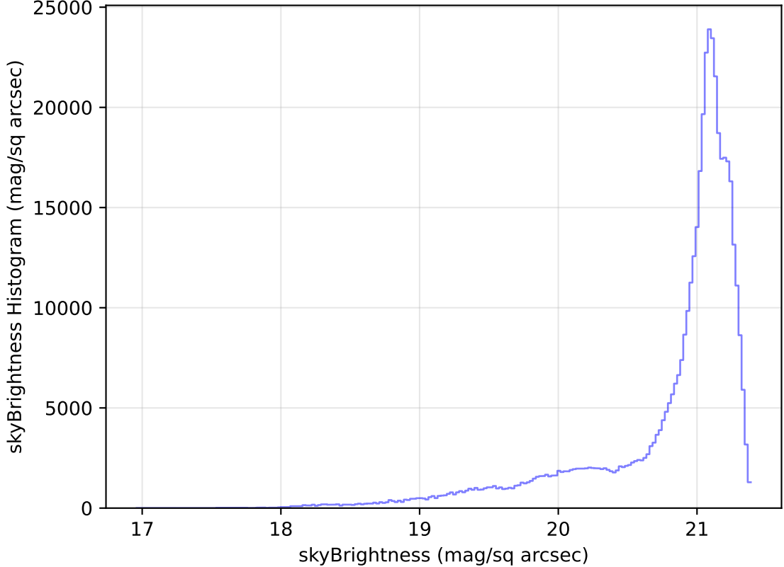
too_elab_heavy_r128_d3_ugrizy_v3.4_10yrs All sky r band: skyBrightness Histogram
