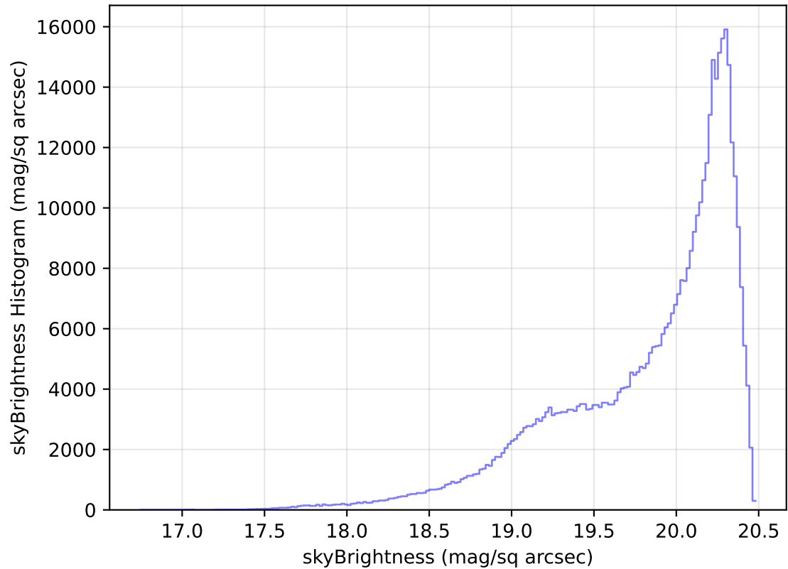
too_elab_heavy_r128_d3_ugrizy_v3.4_10yrs All sky i band: skyBrightness Histogram
