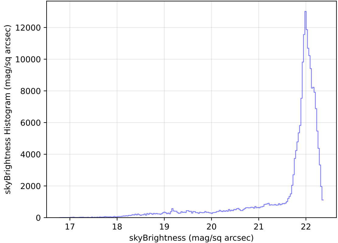
too_elab_heavy_r128_d3_ugrizy_v3.4_10yrs All sky g band: skyBrightness Histogram
