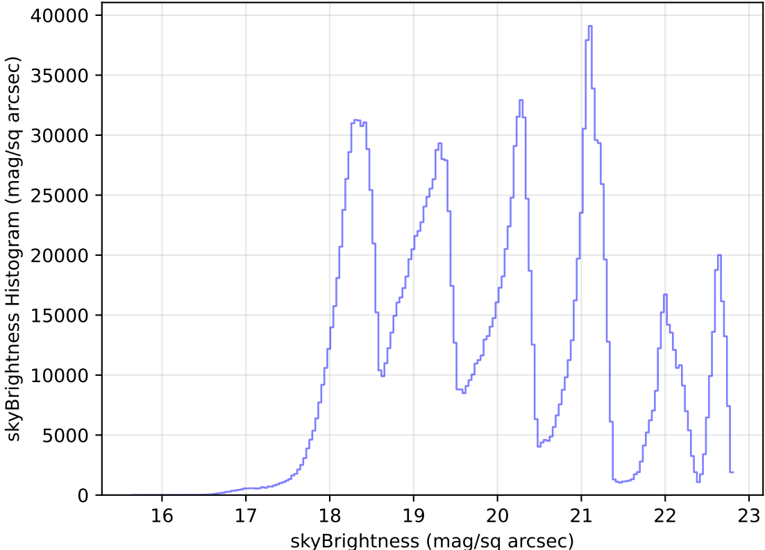
too_elab_heavy_r128_d3_ugrizy_v3.4_10yrs All sky all bands: skyBrightness Histogram
