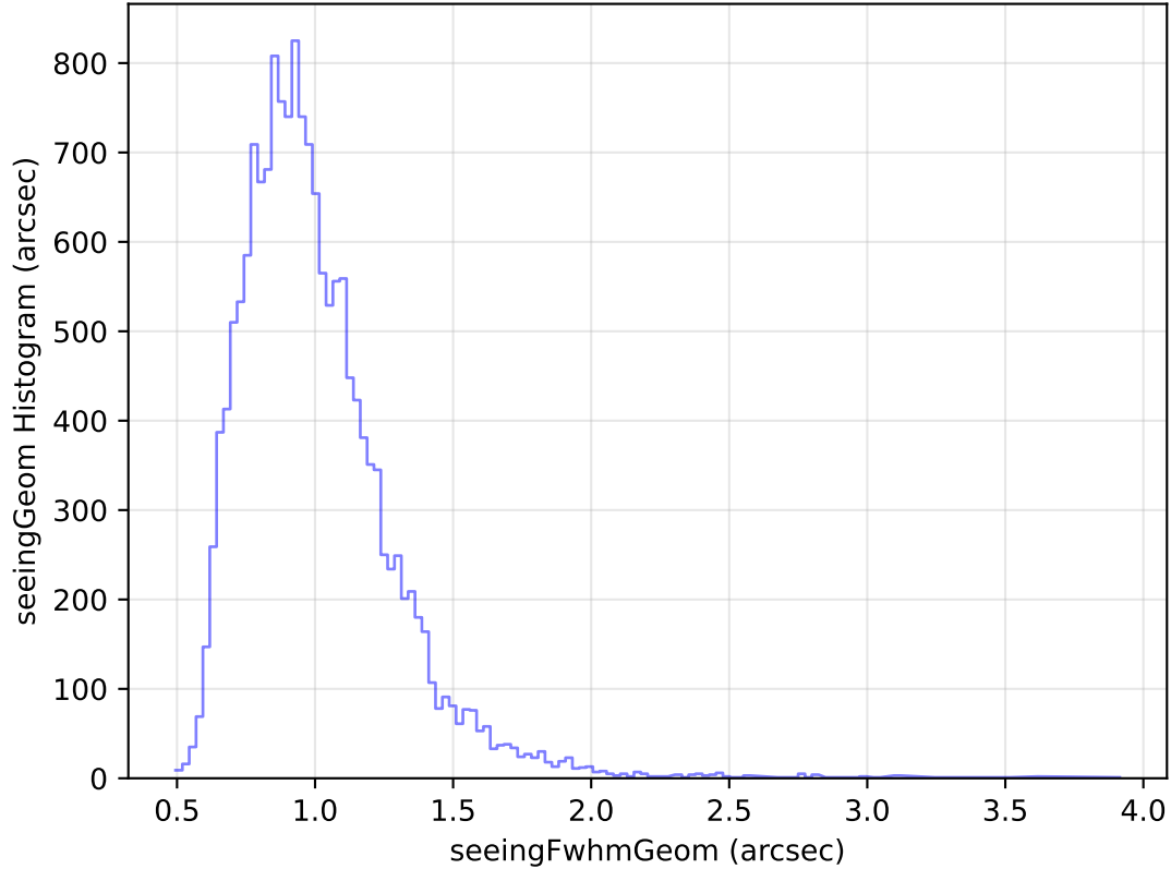
too_elab_heavy_r128_d3_ugrizy_v3.4_10yrs Yr 1 u band: seeingGeom Histogram
