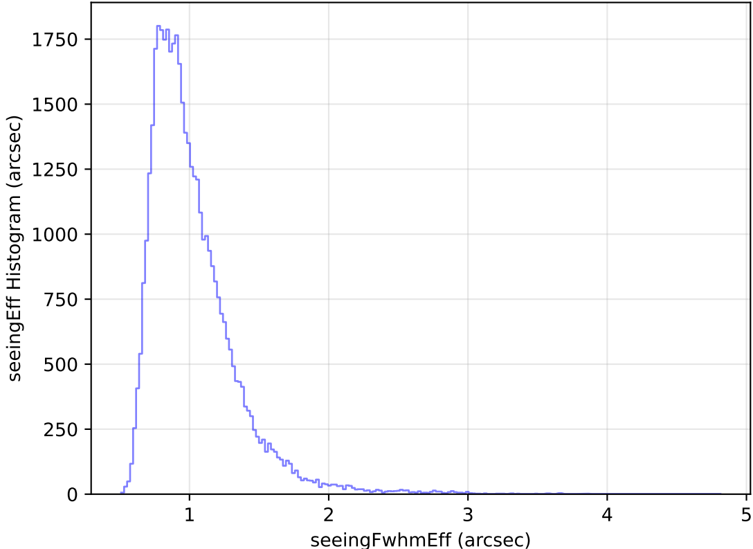
too_elab_heavy_r128_d3_ugrizy_v3.4_10yrs Yr 1 z band: seeingEff Histogram
