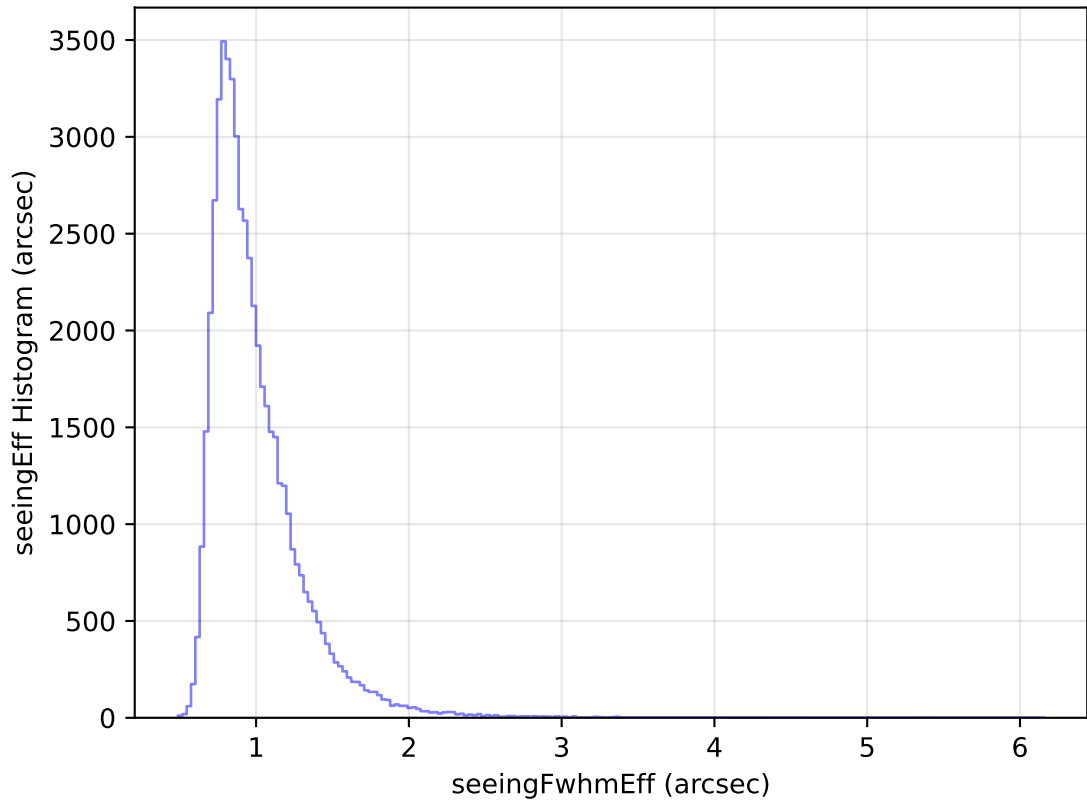
too_elab_heavy_r128_d3_ugrizy_v3.4_10yrs Yr 1 i band: seeingEff Histogram
