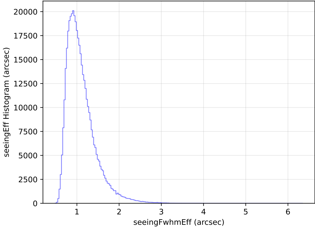
too_elab_heavy_r128_d3_ugrizy_v3.4_10yrs WFD z band: seeingEff Histogram
