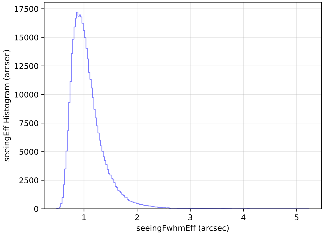
too_elab_heavy_r128_d3_ugrizy_v3.4_10yrs WFD y band: seeingEff Histogram
