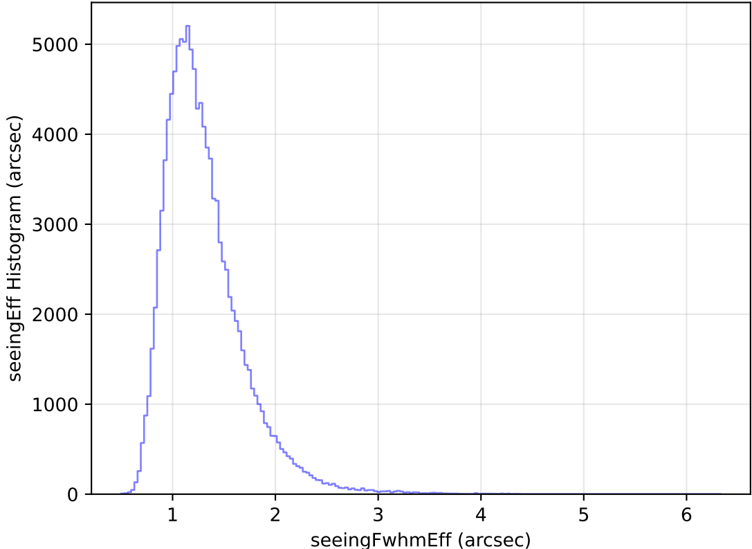
too_elab_heavy_r128_d3_ugrizy_v3.4_10yrs WFD u band: seeingEff Histogram
