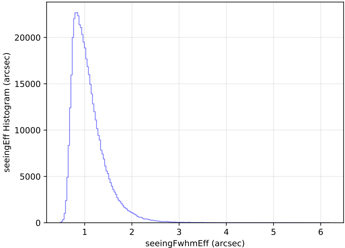
too_elab_heavy_r128_d3_ugrizy_v3.4_10yrs WFD i band: seeingEff Histogram
