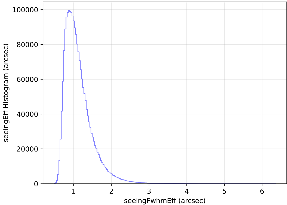
too_elab_heavy_r128_d3_ugrizy_v3.4_10yrs WFD all bands: seeingEff Histogram
