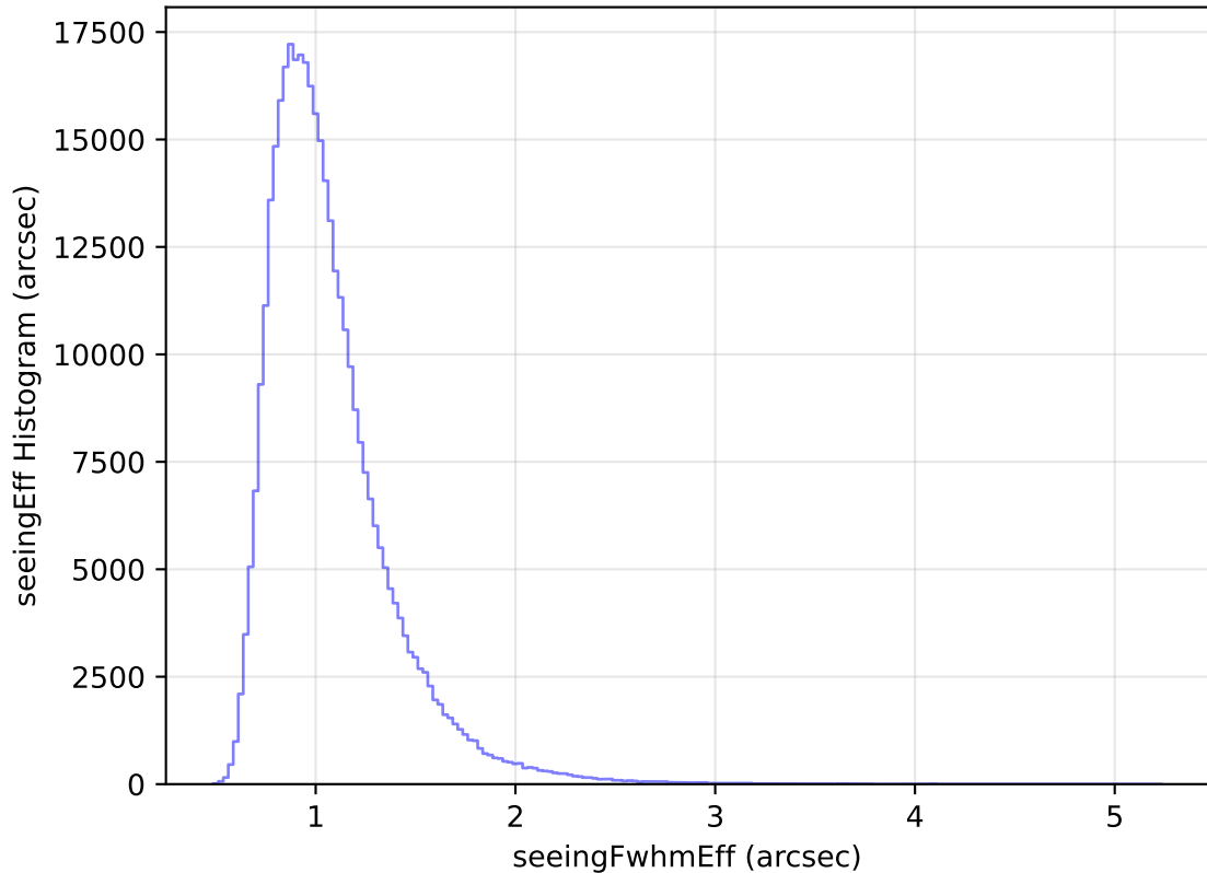
too_elab_heavy_r128_d3_ugrizy_v3.4_10yrs All sky y band: seeingEff Histogram
