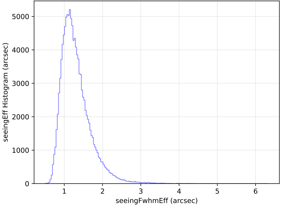
too_elab_heavy_r128_d3_ugrizy_v3.4_10yrs All sky u band: seeingEff Histogram
