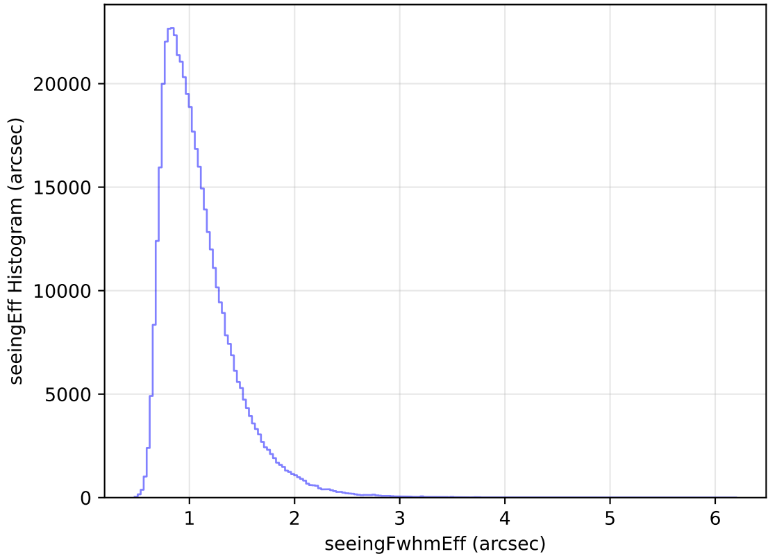
too_elab_heavy_r128_d3_ugrizy_v3.4_10yrs All sky i band: seeingEff Histogram
