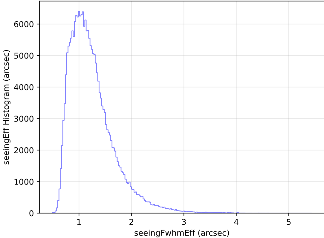
too_elab_heavy_r128_d3_ugrizy_v3.4_10yrs All sky g band: seeingEff Histogram
