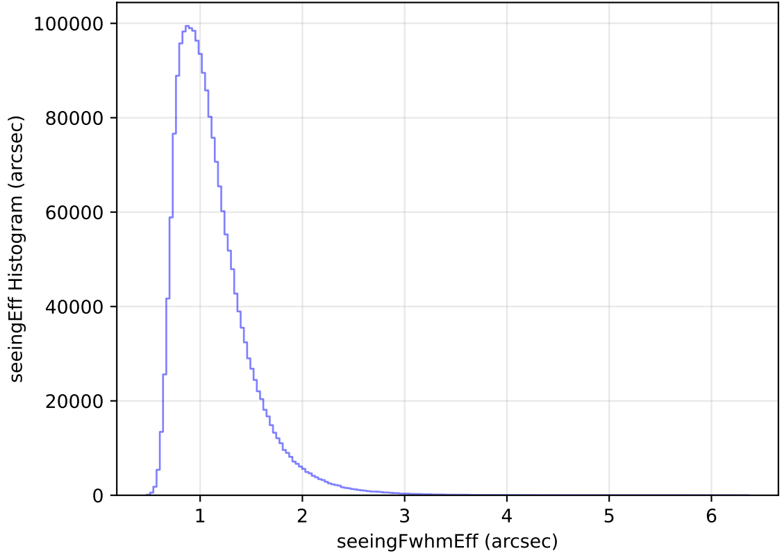
too_elab_heavy_r128_d3_ugrizy_v3.4_10yrs All sky all bands: seeingEff Histogram
