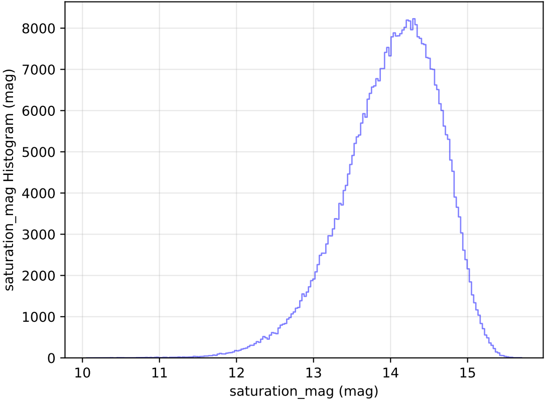
too_elab_heavy_r128_d3_ugrizy_v3.4_10yrs WFD z band: saturation_mag Histogram
