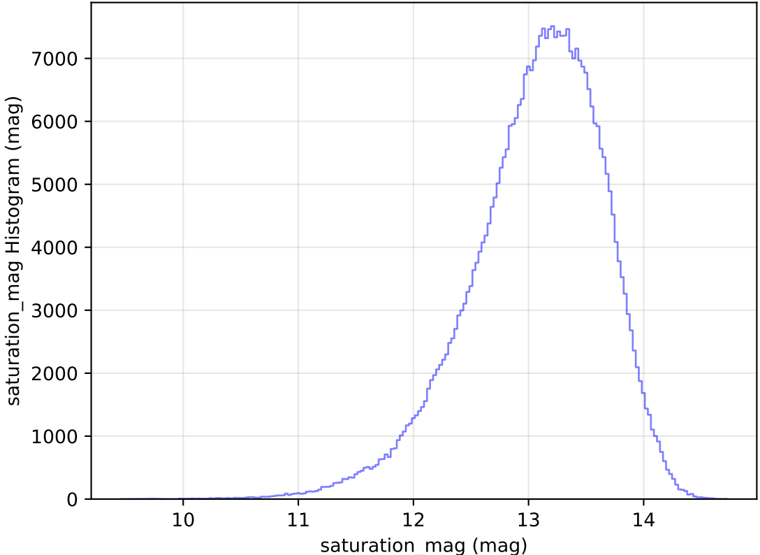
too_elab_heavy_r128_d3_ugrizy_v3.4_10yrs WFD y band: saturation_mag Histogram
