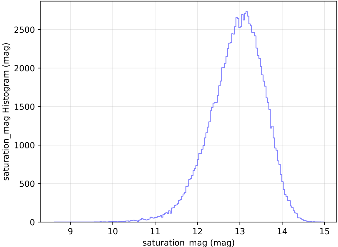
too_elab_heavy_r128_d3_ugrizy_v3.4_10yrs WFD u band: saturation_mag Histogram
