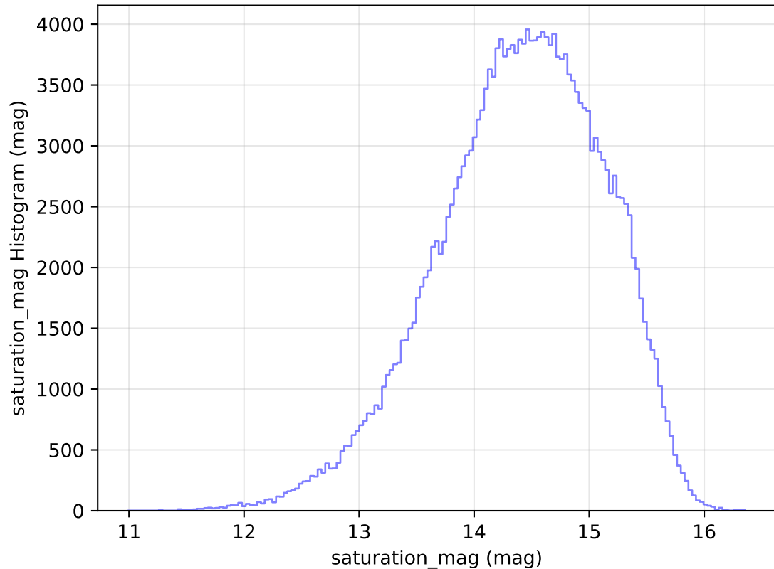
too_elab_heavy_r128_d3_ugrizy_v3.4_10yrs WFD g band: saturation_mag Histogram
