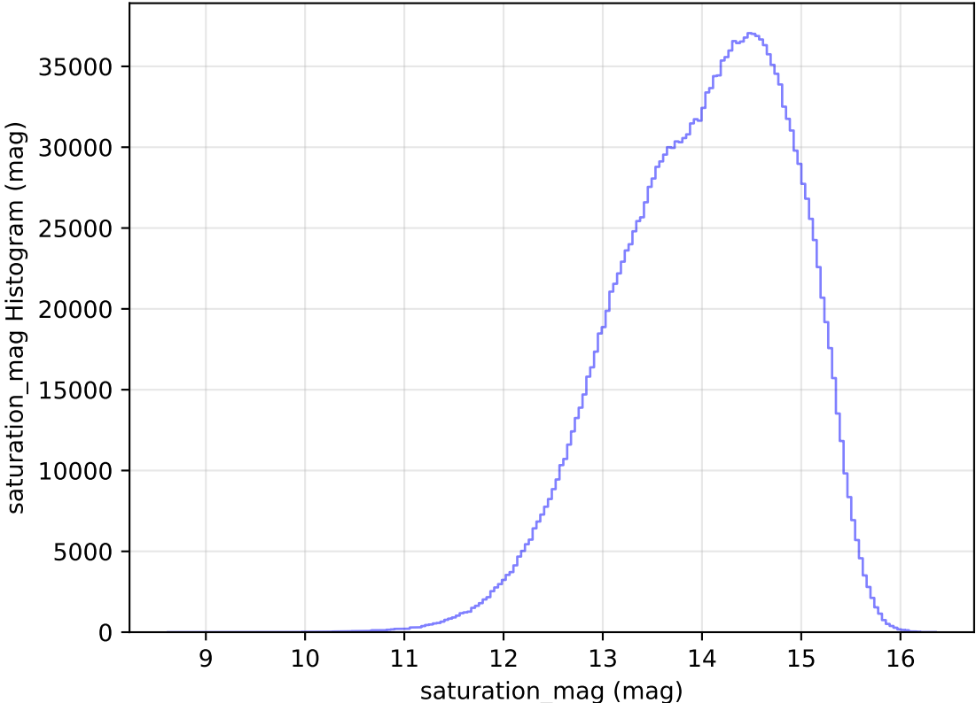
too_elab_heavy_r128_d3_ugrizy_v3.4_10yrs WFD all bands: saturation_mag Histogram
