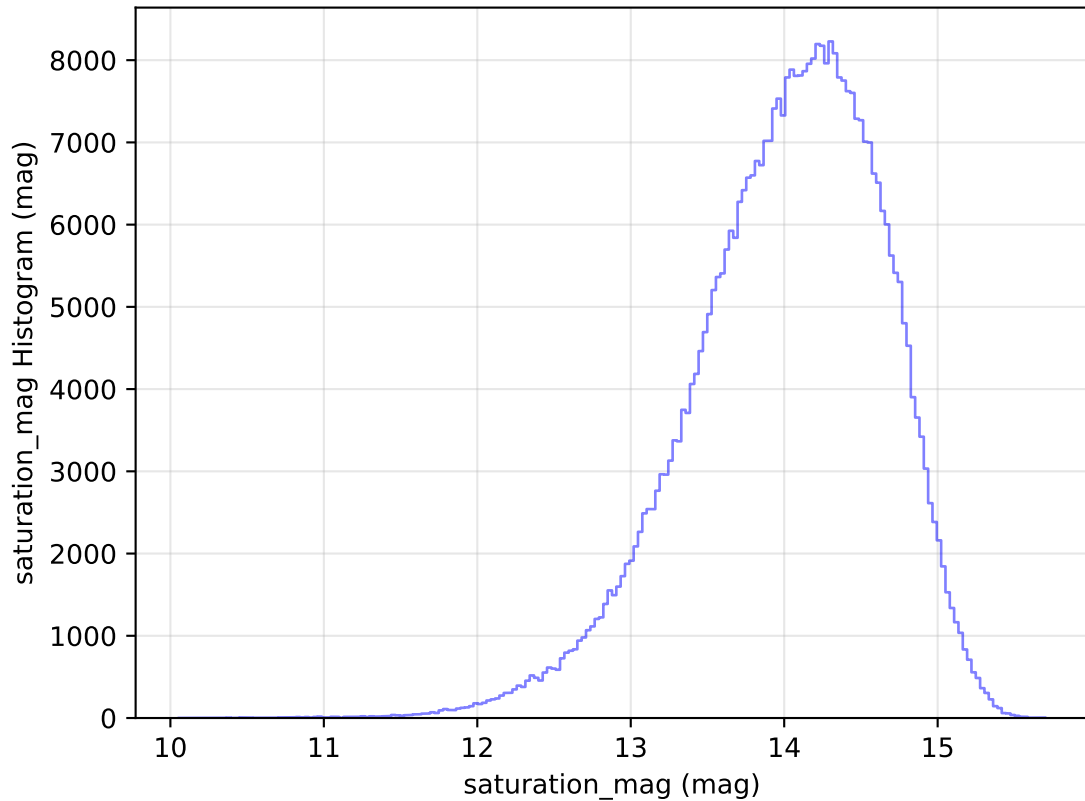
too_elab_heavy_r128_d3_ugrizy_v3.4_10yrs All sky z band: saturation_mag Histogram
