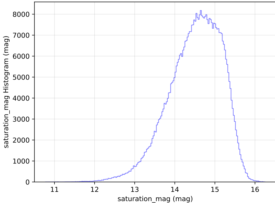
too_elab_heavy_r128_d3_ugrizy_v3.4_10yrs All sky r band: saturation_mag Histogram
