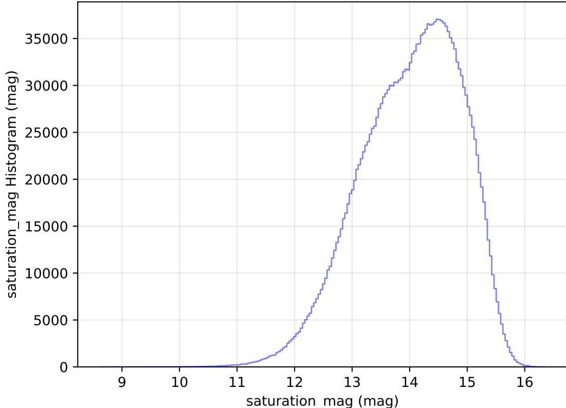
too_elab_heavy_r128_d3_ugrizy_v3.4_10yrs All sky all bands: saturation_mag Histogram
