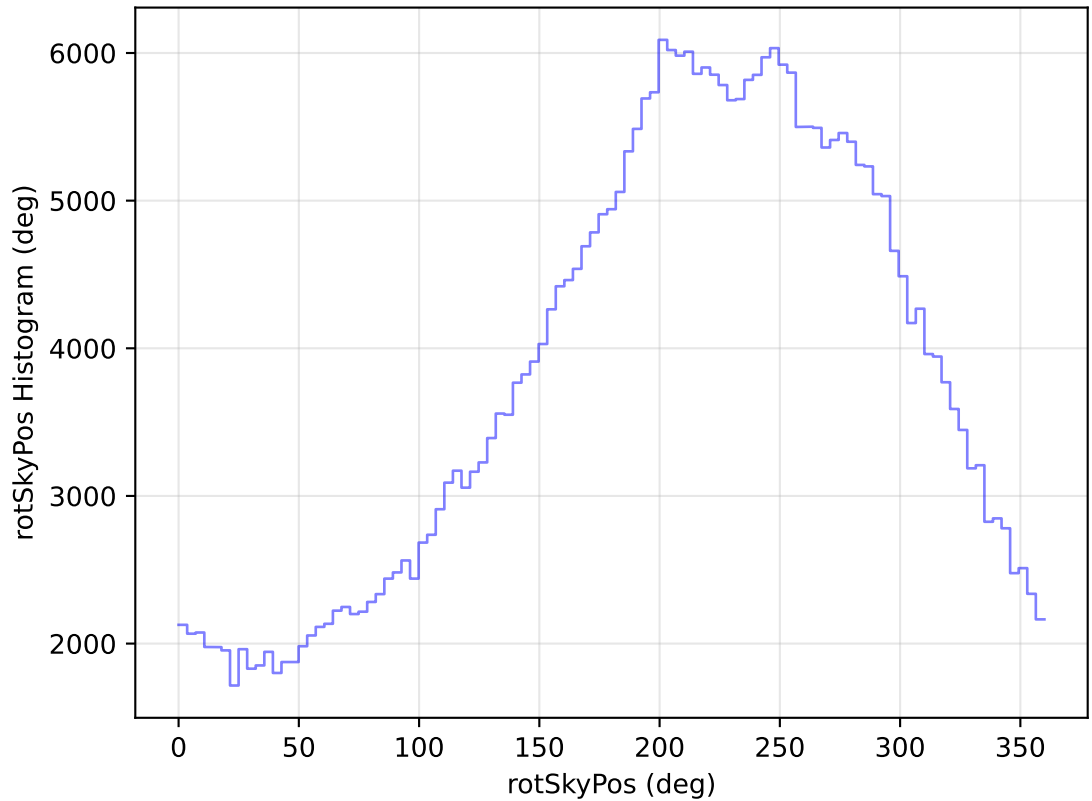
too_elab_heavy_r128_d3_ugrizy_v3.4_10yrs WFD y band: rotSkyPos Histogram
