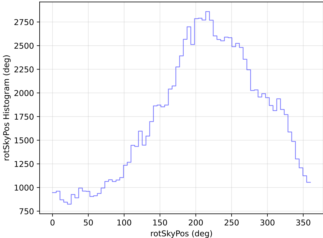
too_elab_heavy_r128_d3_ugrizy_v3.4_10yrs WFD u band: rotSkyPos Histogram
