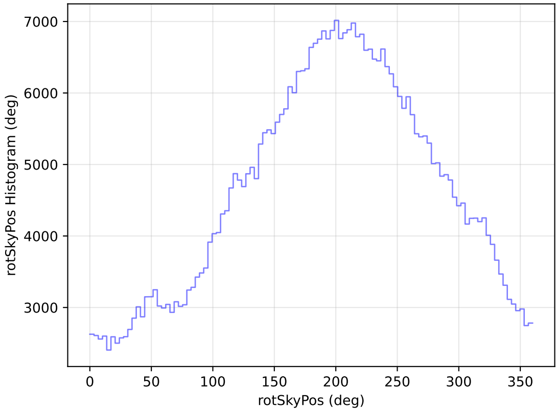
too_elab_heavy_r128_d3_ugrizy_v3.4_10yrs WFD r band: rotSkyPos Histogram
