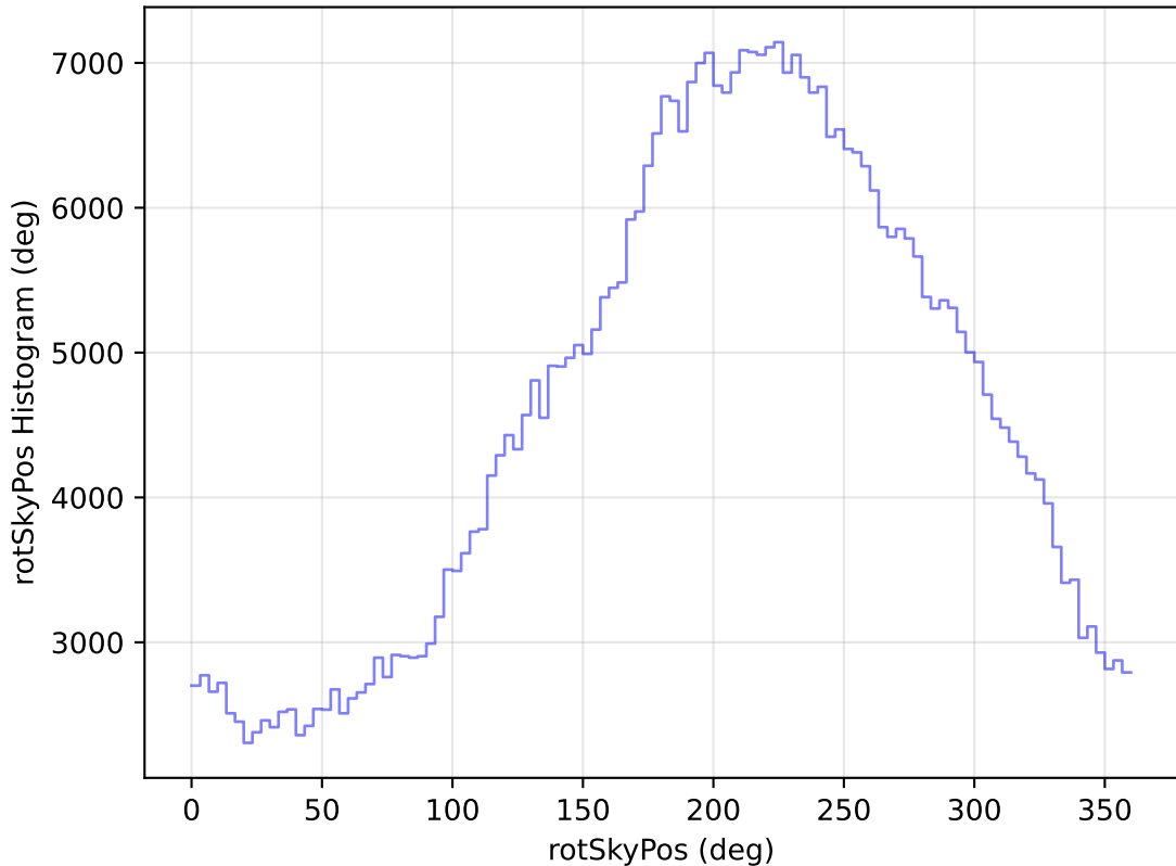
too_elab_heavy_r128_d3_ugrizy_v3.4_10yrs WFD i band: rotSkyPos Histogram
