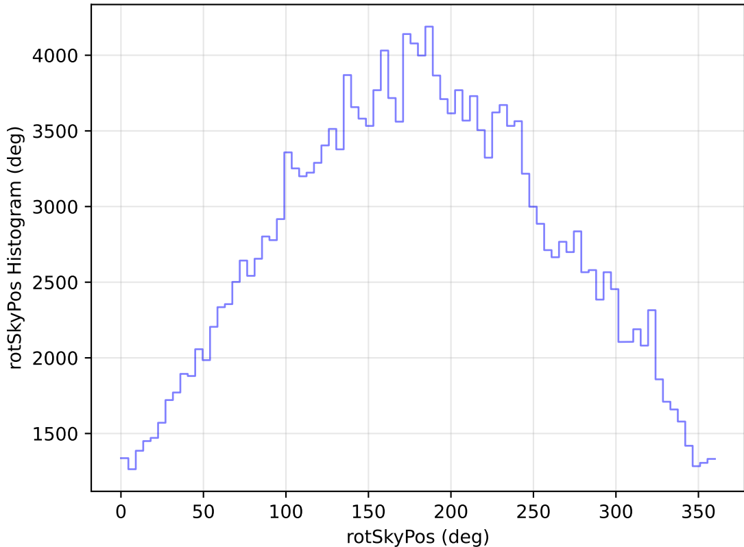
too_elab_heavy_r128_d3_ugrizy_v3.4_10yrs WFD g band: rotSkyPos Histogram
