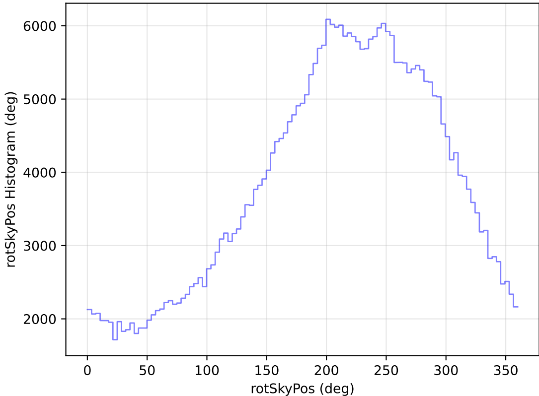
too_elab_heavy_r128_d3_ugrizy_v3.4_10yrs All sky y band: rotSkyPos Histogram
