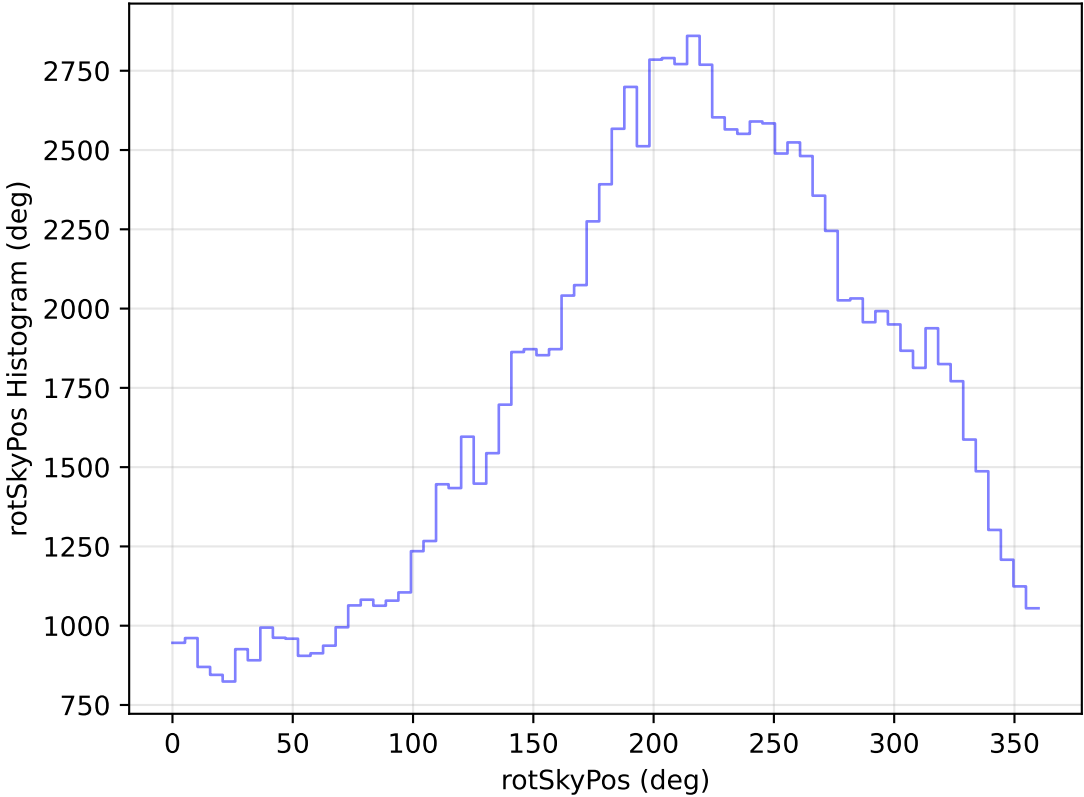
too_elab_heavy_r128_d3_ugrizy_v3.4_10yrs All sky u band: rotSkyPos Histogram
