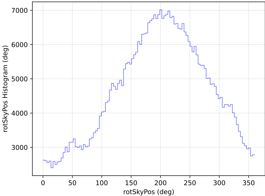
too_elab_heavy_r128_d3_ugrizy_v3.4_10yrs All sky r band: rotSkyPos Histogram
