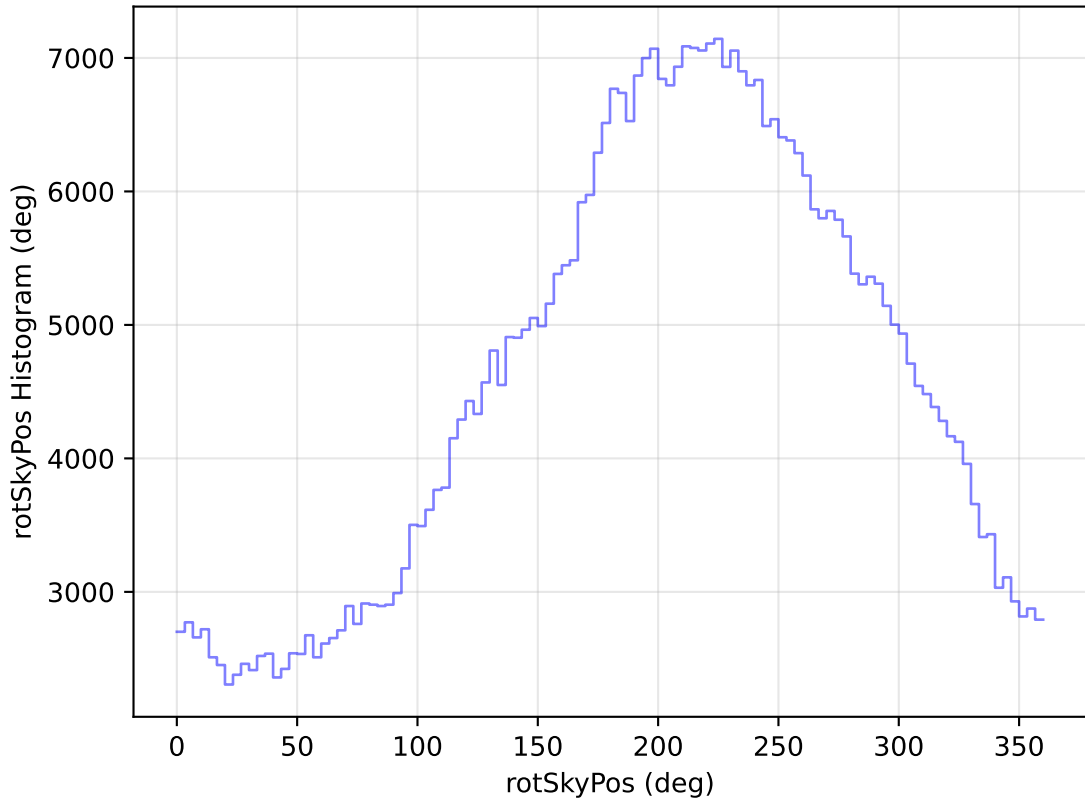
too_elab_heavy_r128_d3_ugrizy_v3.4_10yrs All sky i band: rotSkyPos Histogram
