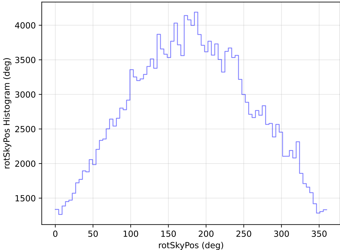
too_elab_heavy_r128_d3_ugrizy_v3.4_10yrs All sky g band: rotSkyPos Histogram
