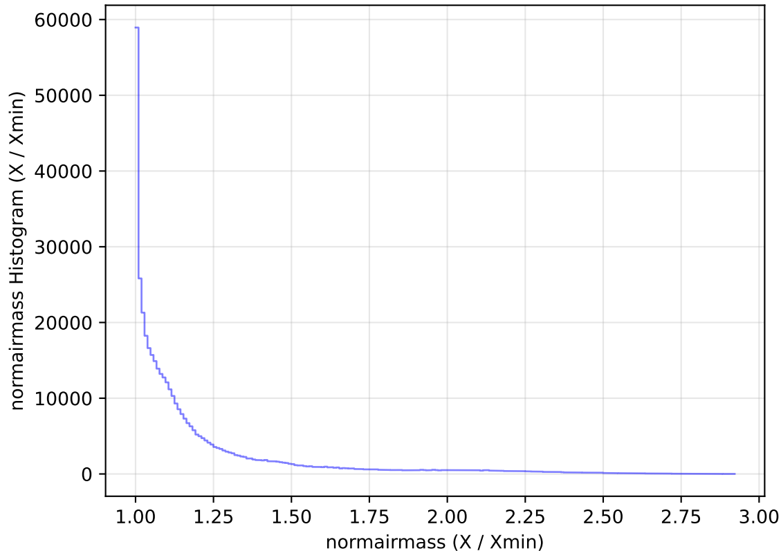
too_elab_heavy_r128_d3_ugrizy_v3.4_10yrs WFD z band: normairmass Histogram
