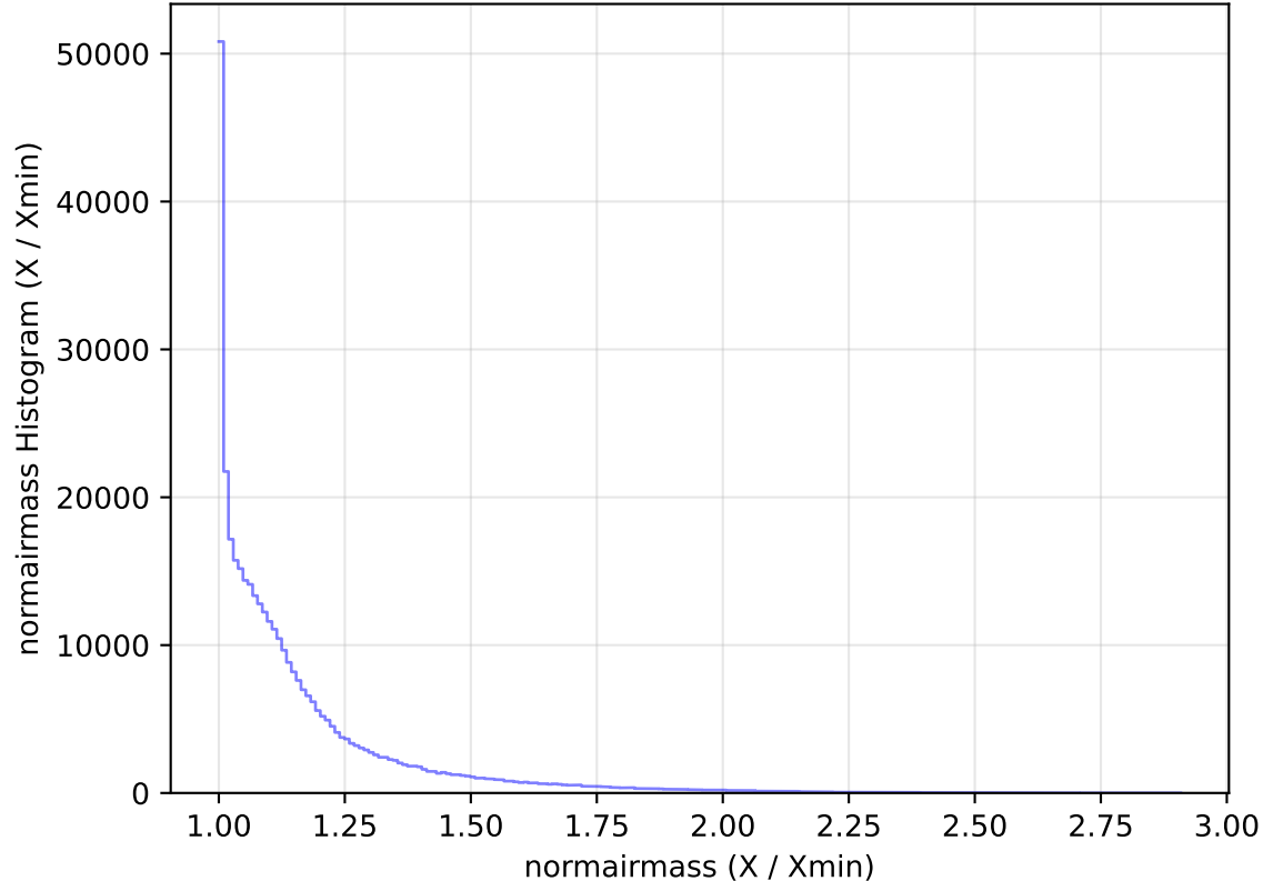
too_elab_heavy_r128_d3_ugrizy_v3.4_10yrs WFD y band: normairmass Histogram
