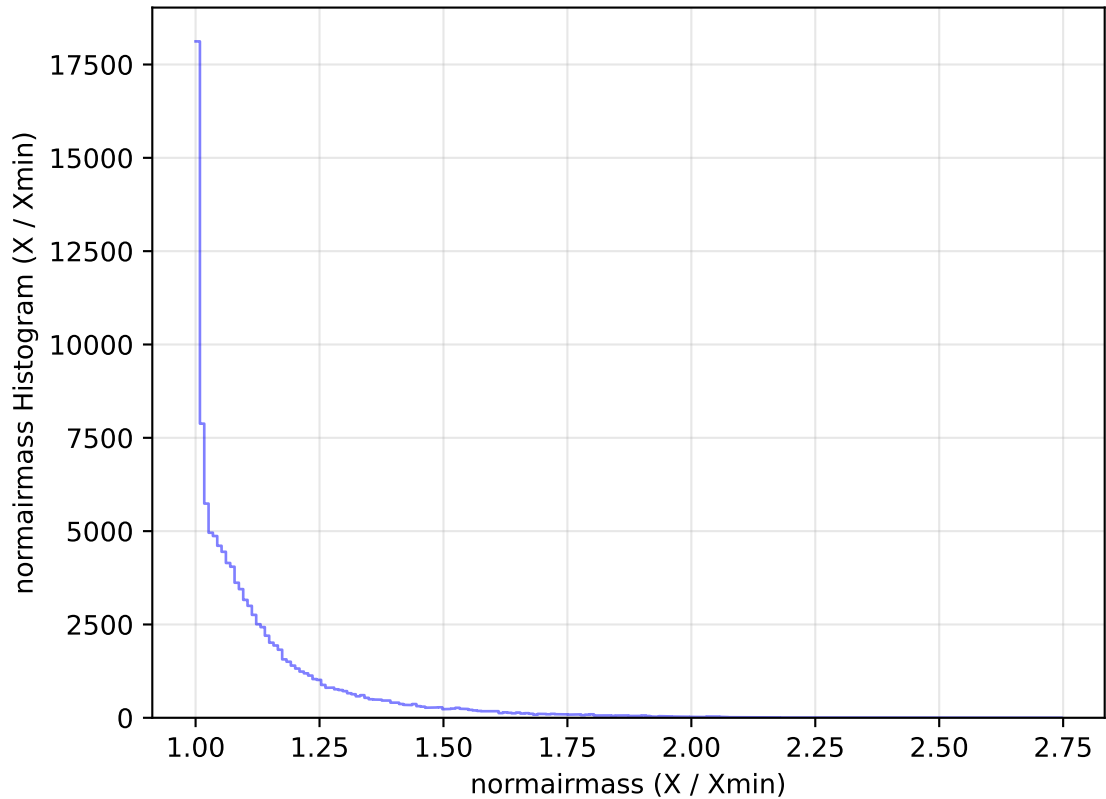
too_elab_heavy_r128_d3_ugrizy_v3.4_10yrs WFD u band: normairmass Histogram
